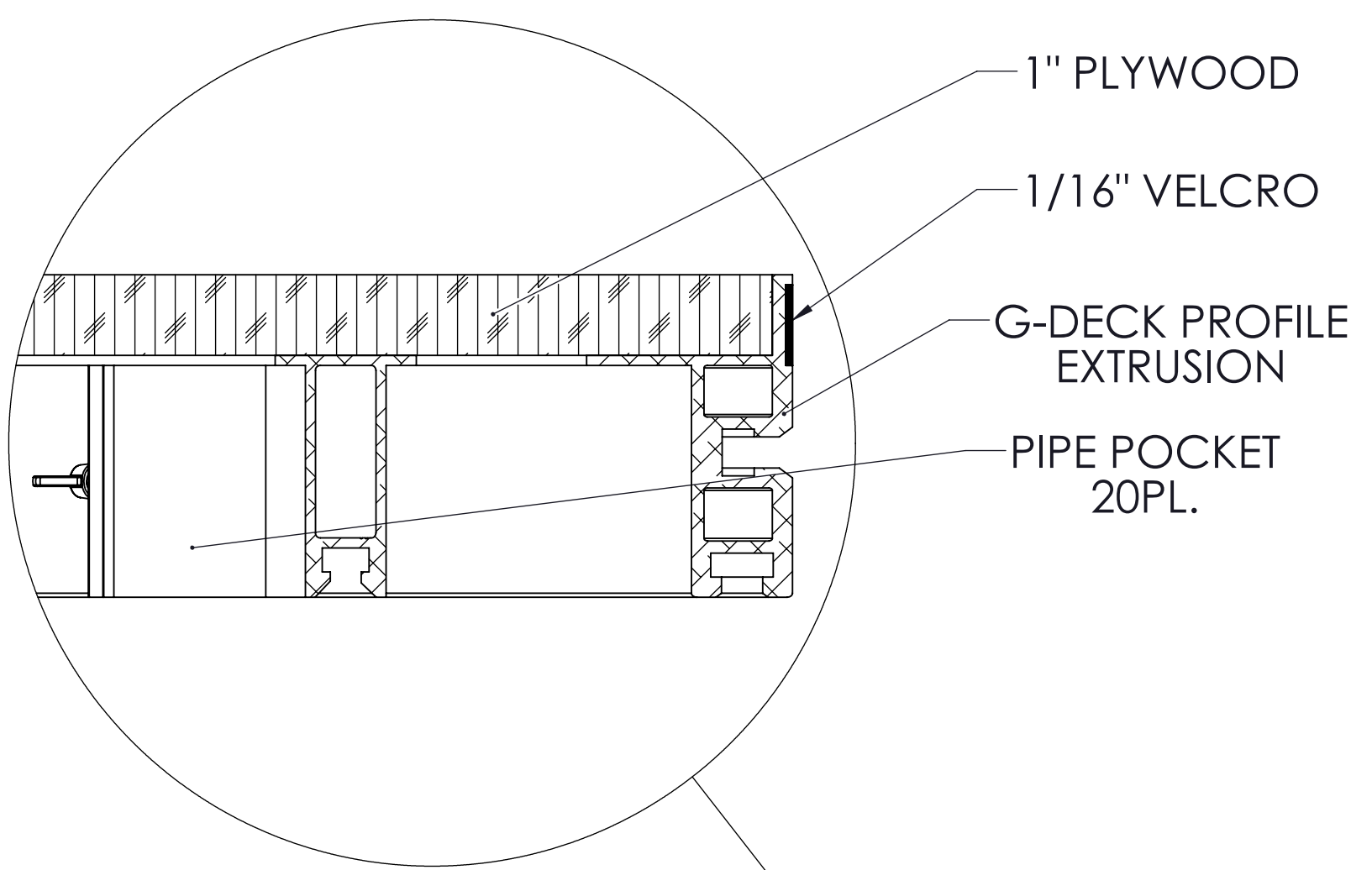
DETAIL H SCALE 1 : 2
