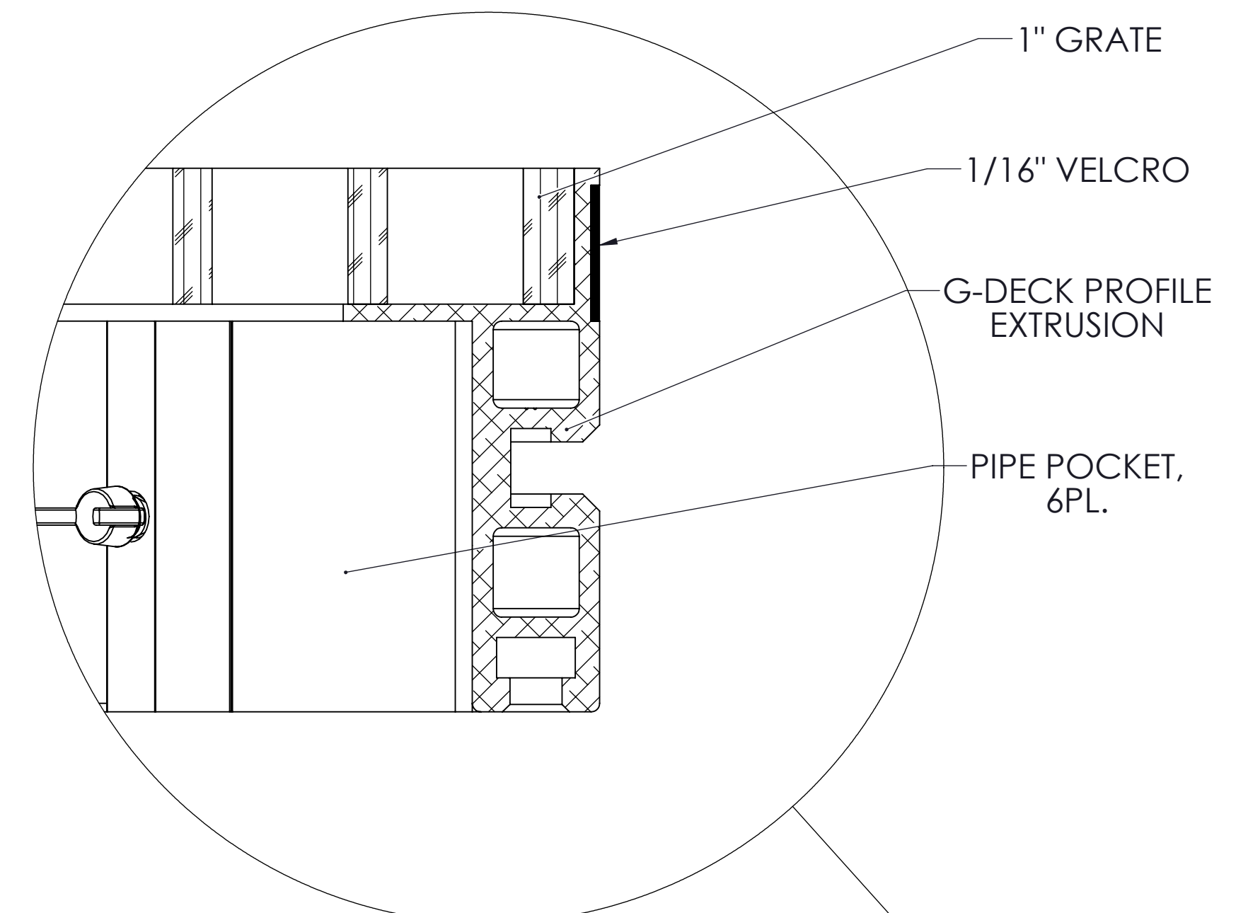
DETAIL B SCALE 1 : 1
