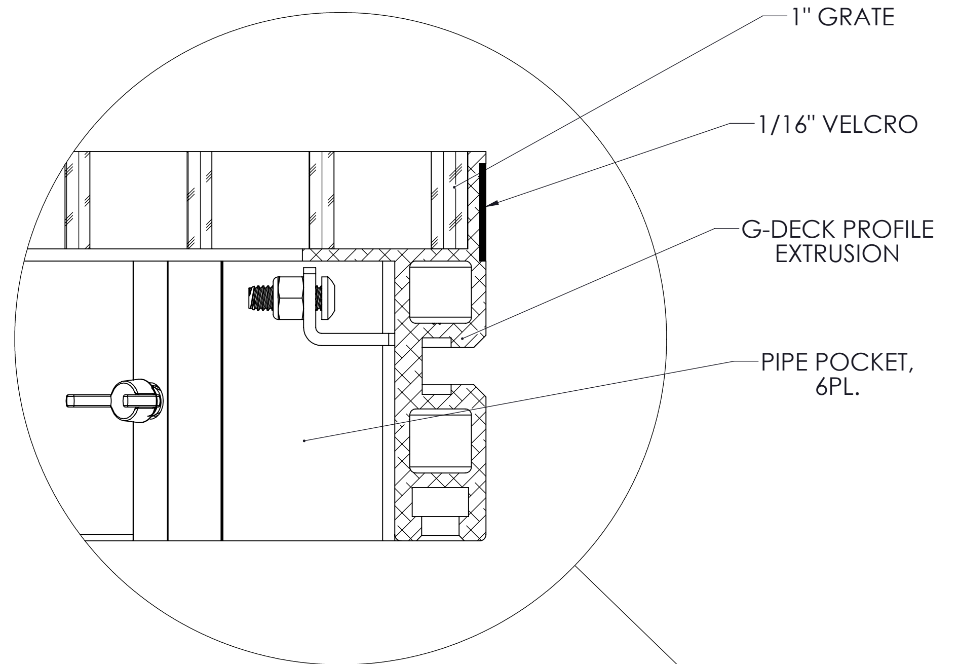
DETAIL B SCALE 1 : 1
